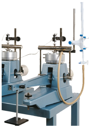
26-WF0338/A Permeability attachment fit to the 26-WF0302 with 26-WF0320 cell
